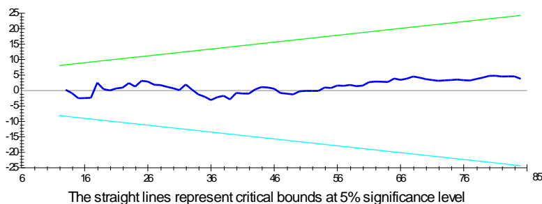
Figure 2. Cumulative Sum of Recursive Residuals (CUSUM)
